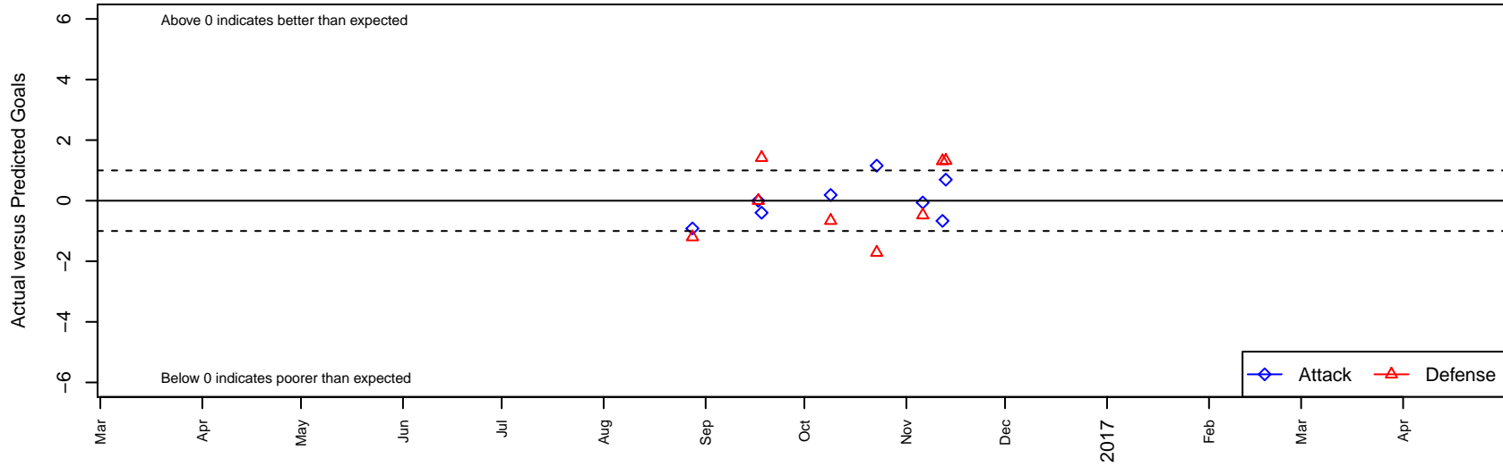
Livermore Fusion SC Maroon G02 Dots are actual minus expected GF (blue circles) and GA (red triangles). Blue line is smoothed change in attack strength. Red is smoothed change in defense strength.
